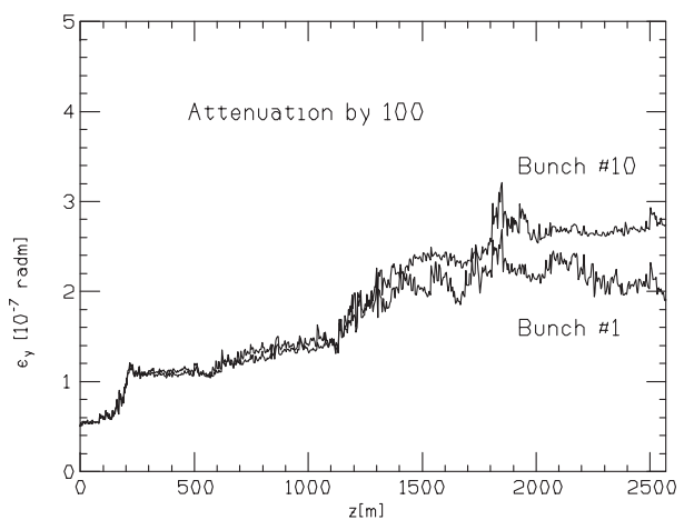
Figure 2: 10th bunch emittance growth with RFQs (1st bunch growth as reference).
